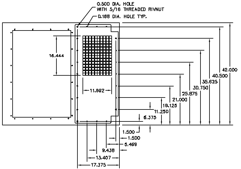
BOTTOM OF 2 CARTRIDGE COLLECTOR
