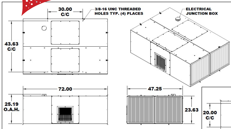
HORIZONTAL STACK CONFIGURATION
